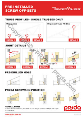
Poster #3 SpeedTruss - "Pre-Installed Screw Off-Sets [Page 1]"
