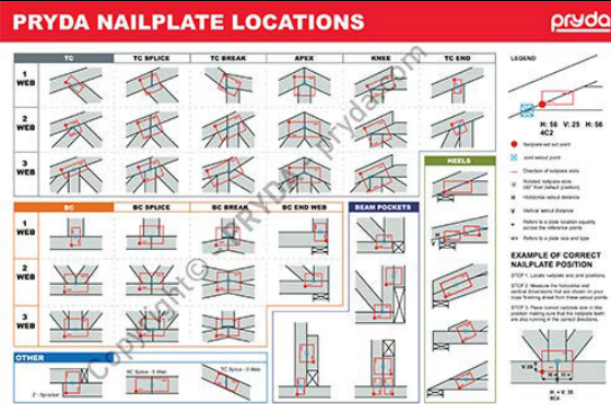
Poster #1 "Pryda Nailplate Locations"
